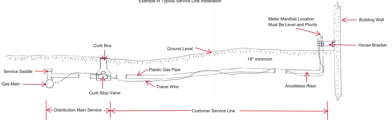
Example of Typical Service Line Installation
